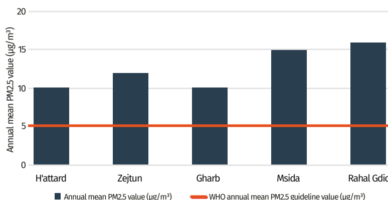
FIGURE 8: Annual mean PM_{2.5} in Malta cities, for which data were available, compared with the WHO guideline value of PM_{2.5} of 5 \mu\text{g}/\text{m}^3 . Source: Ambient Air Pollution Database, WHO, 2018. A standard conversion has been used on some data points, see source for further details (15)
