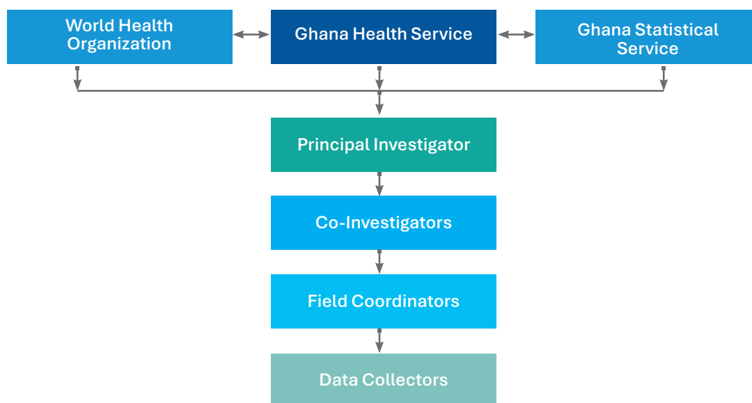
Figure 2.7.1.1: Implementation Structure
