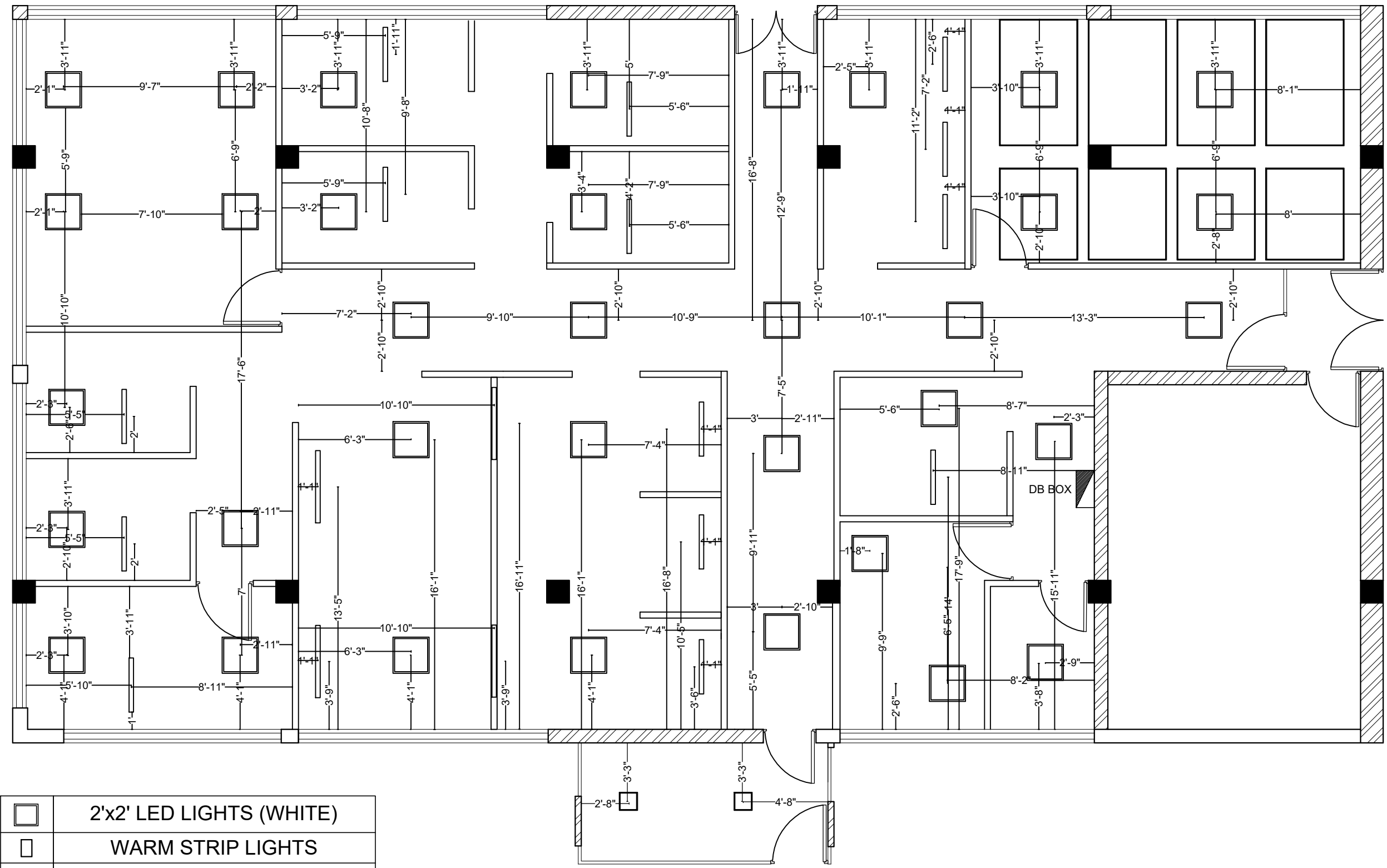
LIGHTS LAYOUT PLAN SCALE= 1:100
