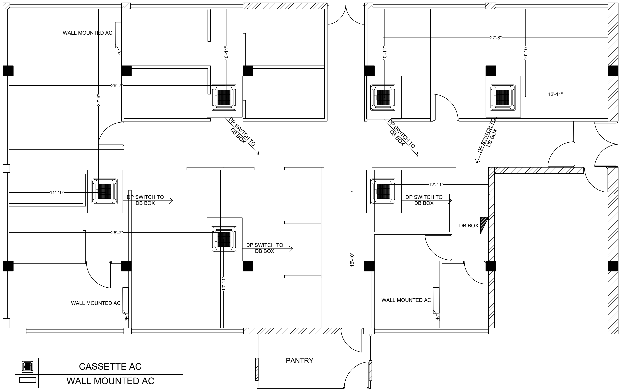
AC LAYOUT PLAN SCALE= 1:100
