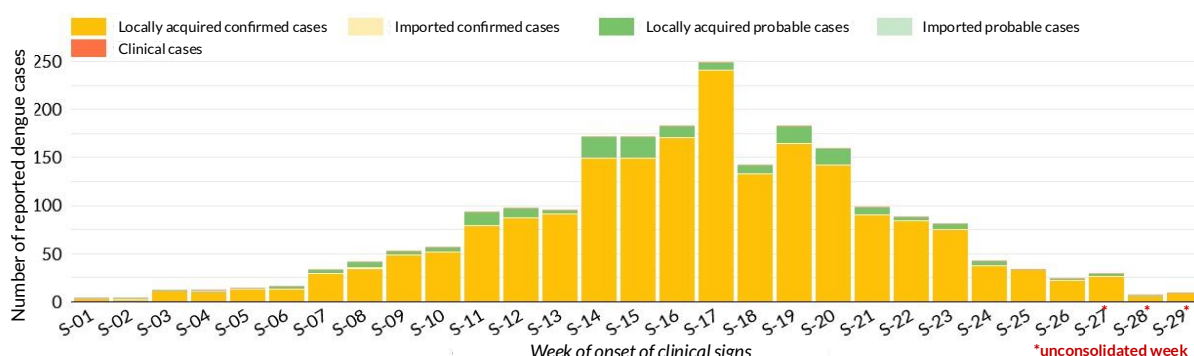
Figure 9: Dengue cases reported by week from 1 January to 19 July 2026 in New Caledonia
